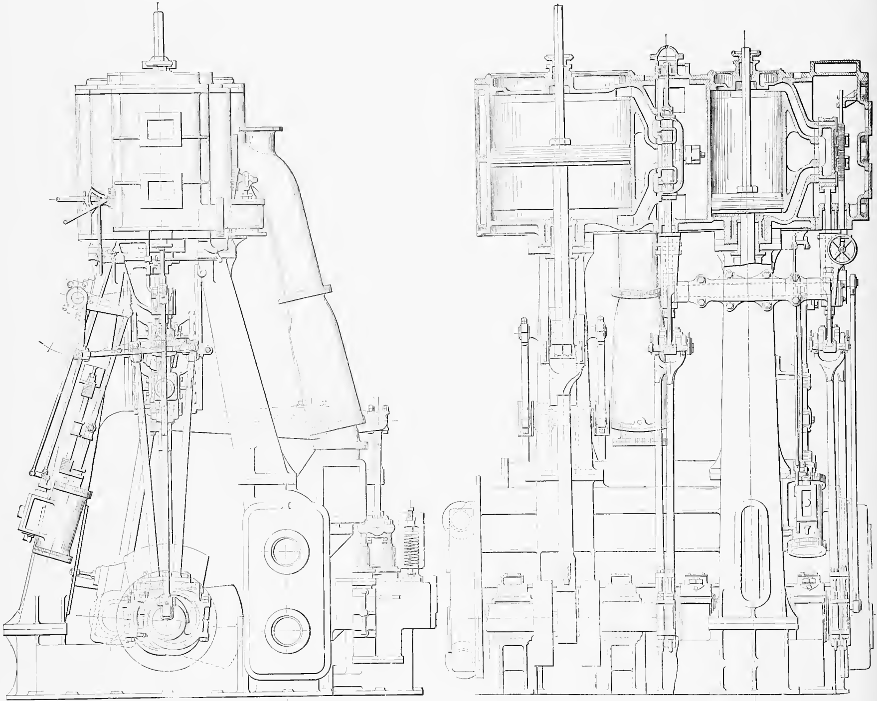
COMPOUND ENGINE OF TUG EDWIN H. MEAD.—Built by T. S. Marvel & Co., Newburgh, N. Y., for the Cornell Steamboat Co., Rondout, N. Y.
